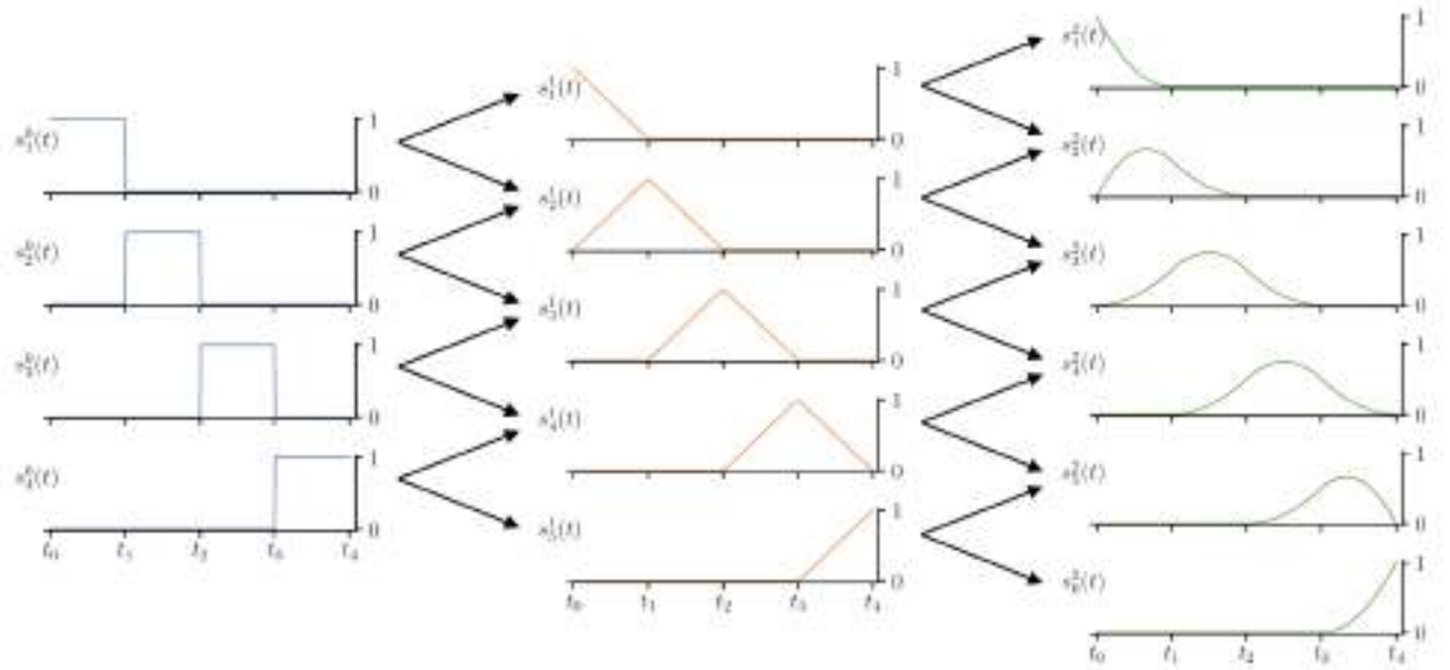
Figure A. Generation of B-spline basis elements (orders 0, 1, 2)
